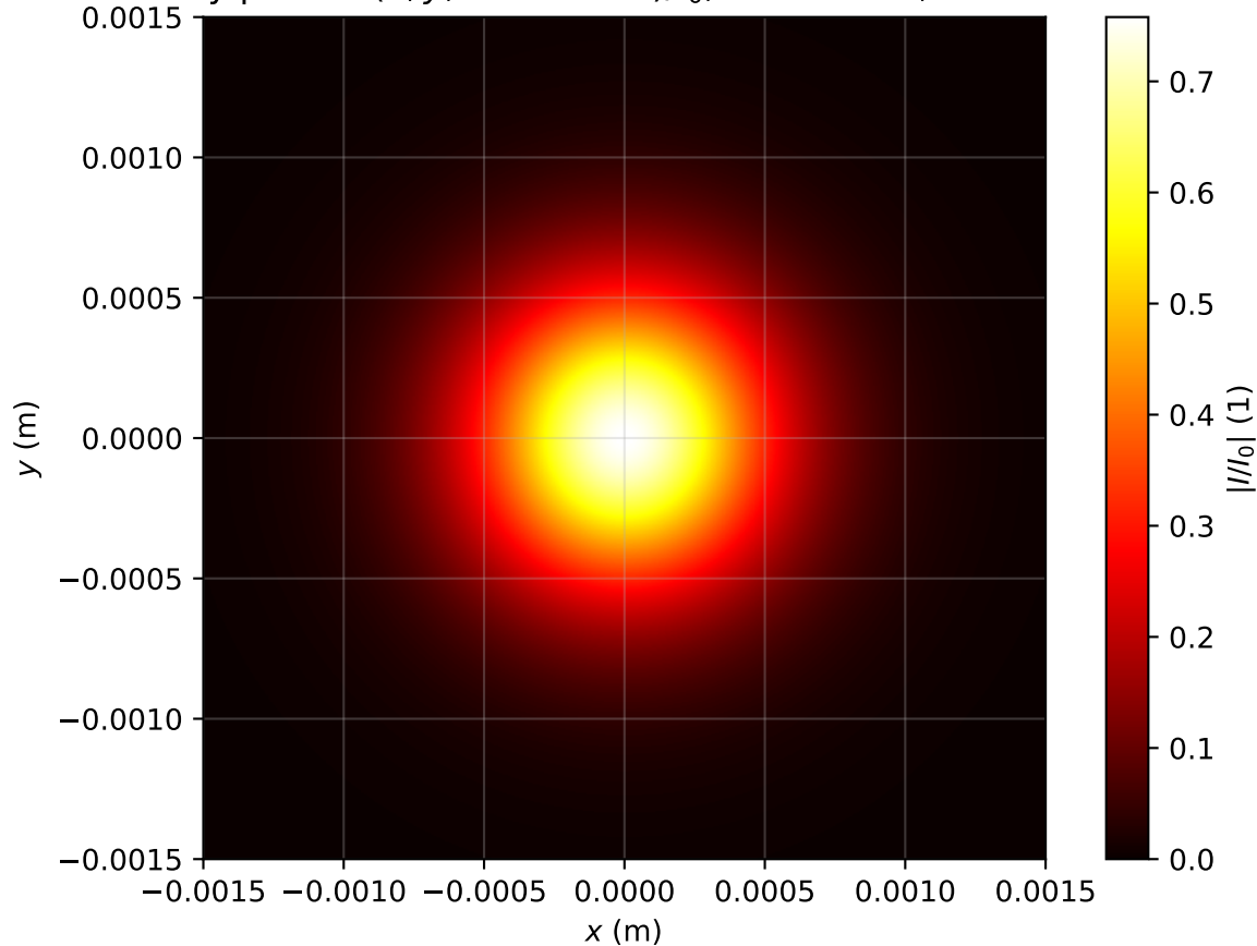
Intensity profile I(x, y, z = 2.229m)/I_0 , Pin=0.5Pcr, artificial time
